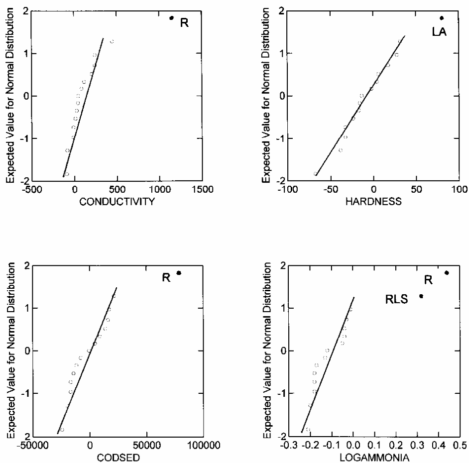
Figure E-13. Significant main and interacting factors for common constituent concentrations in water found in telecommunication manholes.
