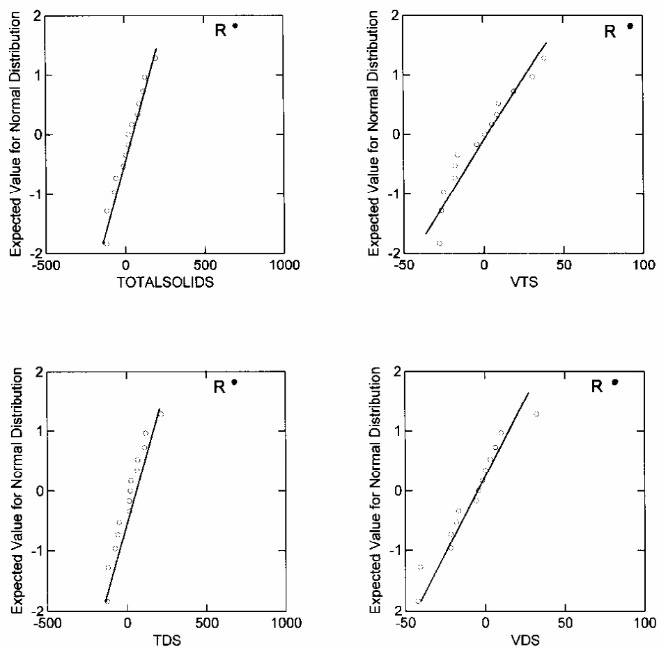
Figure E-12. Significant main and interacting factors for solids concentrations in water found in telecommunication manholes.
