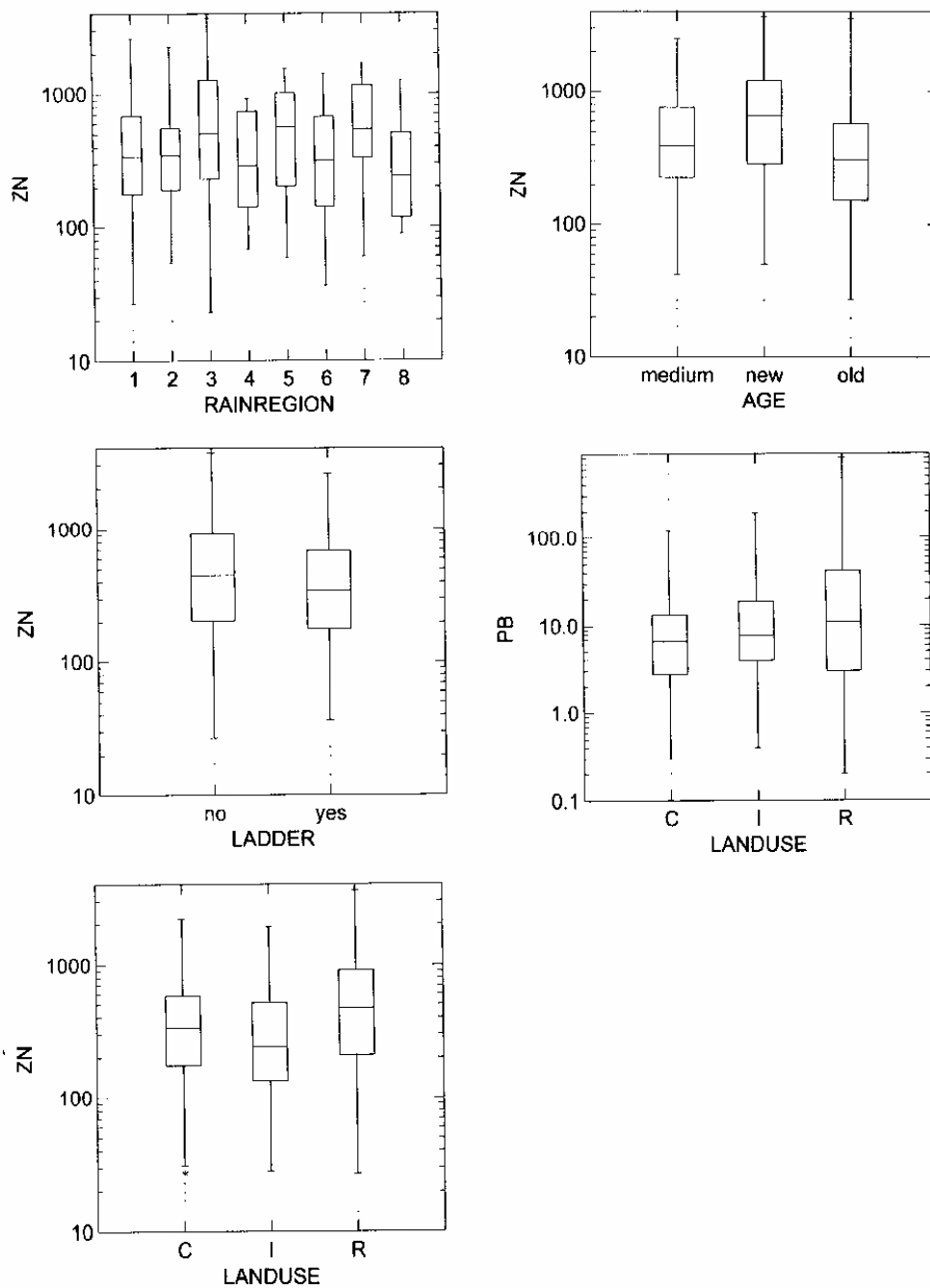
Figure E-9. Statistically significant groupings for “zinc” concentrations found in water from telecommunication manholes.
